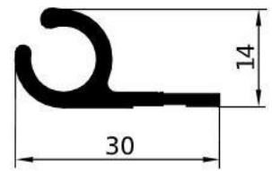
GA1548 – gr/ml 283 L/mm.7000 PACCO / 10 BARRE
