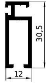
GA1538 – gr/ml 324 L/mm.6500 PACCO / 10 BARRE
