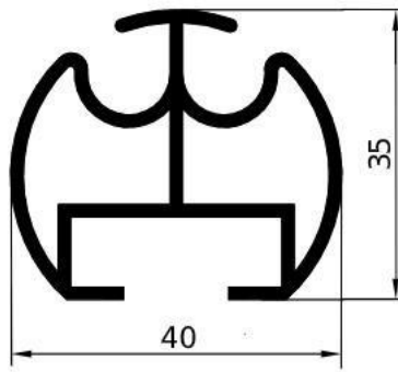
GA1558 – gr/ml 801 L/mm.7000 PACCO / 5 BARRE
