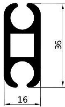
GA1599 – gr/ml 694 L/mm.7000 PACCO / 5 BARRE
