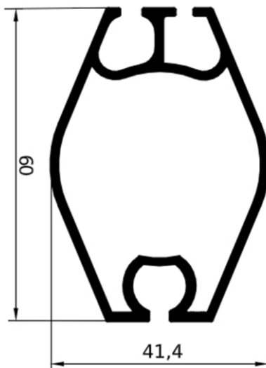
GA1528 – gr/ml 852 L/mm. 7000 PACCO / 3 BARRE
