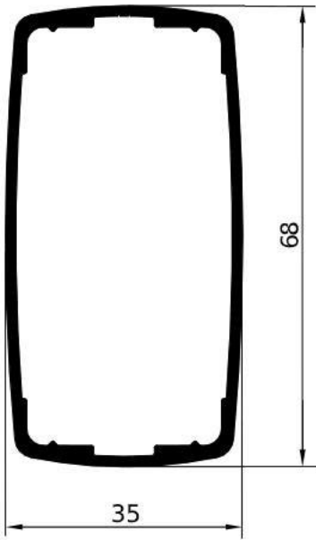
GA1508 – gr/ml 906 L/mm.7000 PACCO / 2 BARRE
