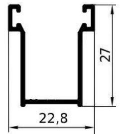
GA1626 – gr/ml 218 L/mm.6500 PACCO / 10 BARRE
