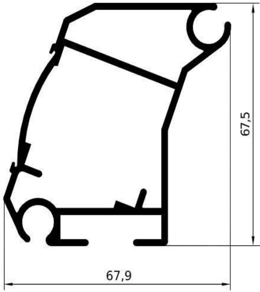
GA1004 – gr/ml 1453 L/mm. 4000-5000 6000-7000 PACCO / 2 BARRE
