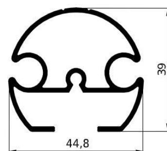
GA1055 – gr/ml 679 L/mm.5000-7000 PACCO / 5 BARRE
