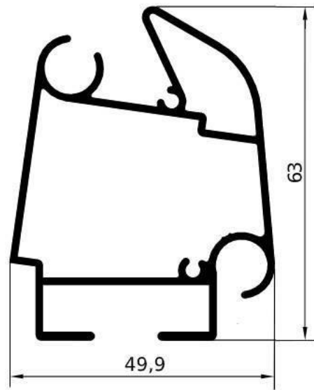
GA1050 – gr/ml 1037 L/mm. 4000-5000 6000-7000 PACCO / 2 BARRE
