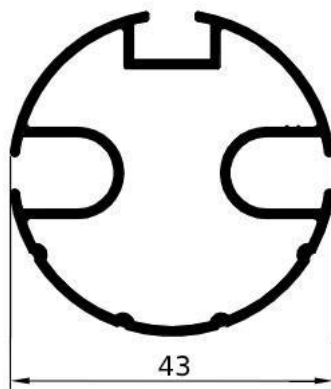
GA1525 – gr/ml 662 L/mm.4000-5000- 6000-7000 PACCO / 5 BARRE
