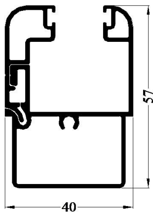
AC135 – Kit Guida Zip L/ mm.6000 PACCO / 1 BARRA
