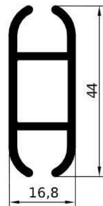
GA1576 – gr/ml 582 L/mm.6000 PACCO / 5 BARRE
