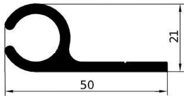
GA1627 – gr/ml 715 L/mm.6000 PACCO / 6 BARRE
