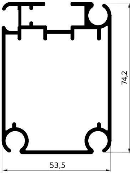
GA1602 – gr/ml 1350 L/mm.5000 - 7000 PACCO / 2 BARRE
