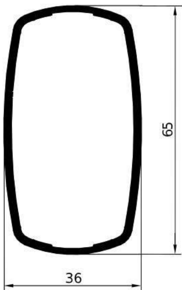
GA1511 – gr/ml 899 L/mm.7000 PACCO / 2 BARRE
