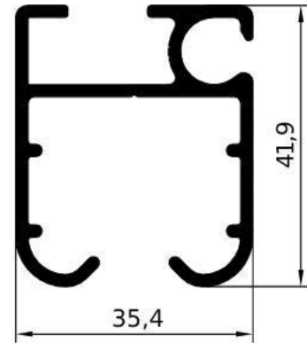
GA1681 – gr/ml 820 L/mm.5000 – 7000 PACCO / 5 BARRE
