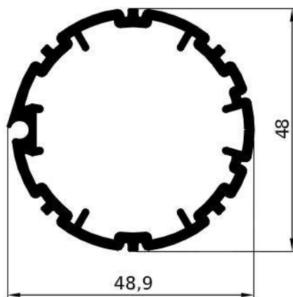
GA1651 – gr/ml 980 L/mm.6000 PACCO / 5 BARRE
