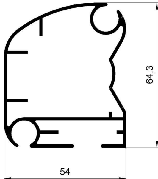
GA1053 – gr/ml 1196 L/mm. 4000-5000 6000-7000 PACCO / 2 BARRE
