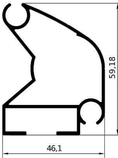
GA1510 – gr/ml 800 L/mm. 4000-5000 6000-7000 PACCO / 2 BARRE
