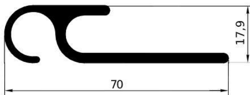
GA1552 – gr/ml 863 L/mm.6500 PACCO / 4 BARRE
