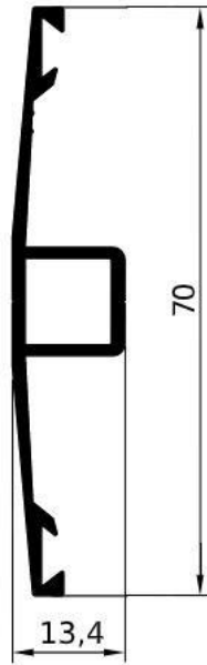
GA1630 – gr/ml 433 L/mm.6000 PACCO / 10 BARRE
