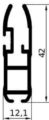
GA1650 – gr/ml 417 L/mm.6000 PACCO / 5 BARRE
