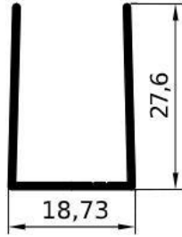
GA1596 – gr/ml 278 MIN KG.500
