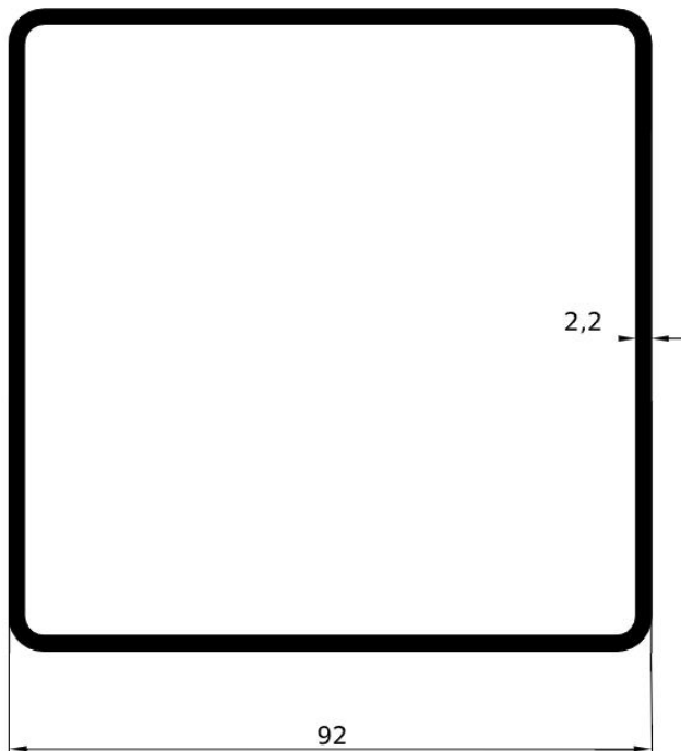
GA1502 – gr/ml 2095 L/mm.4500-5100
