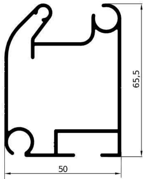
GA1515 – gr/ml 1078 L/mm. 4000-5000 6000-7000 PACCO / 2 BARRE
