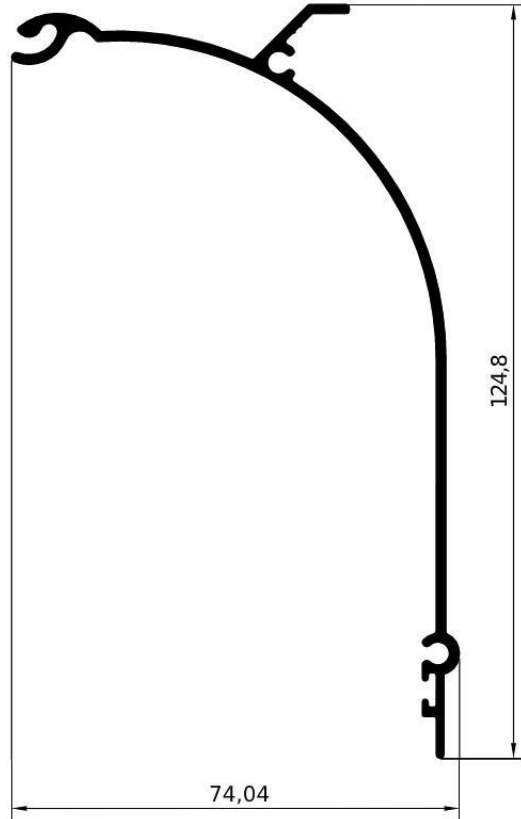
GA1621 – gr/ml 920 L/mm.5000-7000 PACCO / 2 BARRE
