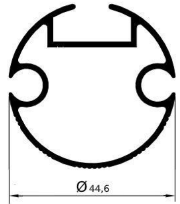
GA1512 – gr/ml 702 L/mm.5000-6000-7000 PACCO / 5 BARRE
