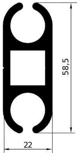
GA1052 – gr/ml 1425 L/mm.7000 PACCO / 4 BARRE
