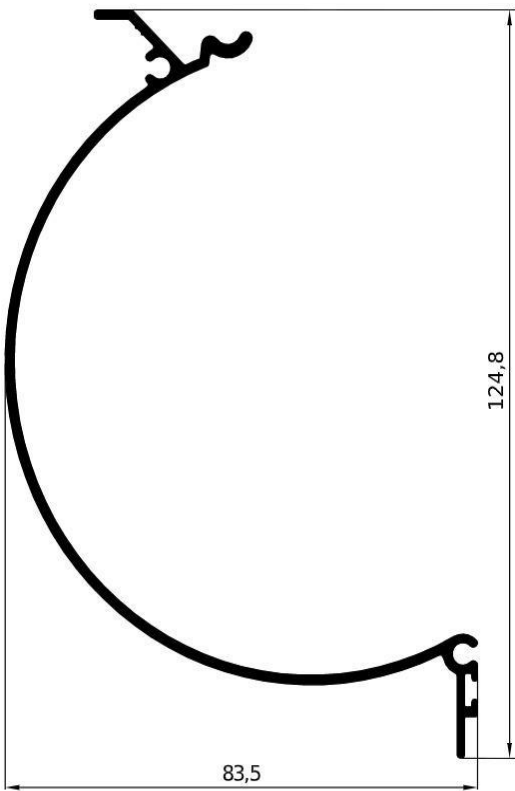
GA1622 – gr/ml 1028 L/mm.5000-7000 PACCO / 2 BARRE
