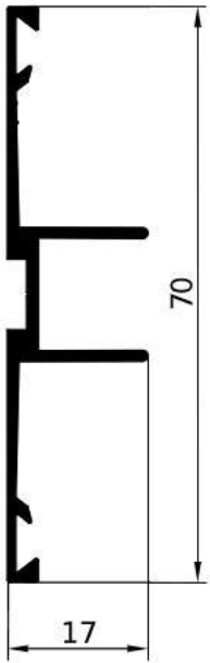
GA1629 – gr/ml 411 L/mm.6000 PACCO / 10 BARRE
