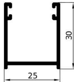
GA1625 – gr/ml 303 L/mm.6500 PACCO / 10 BARRE
