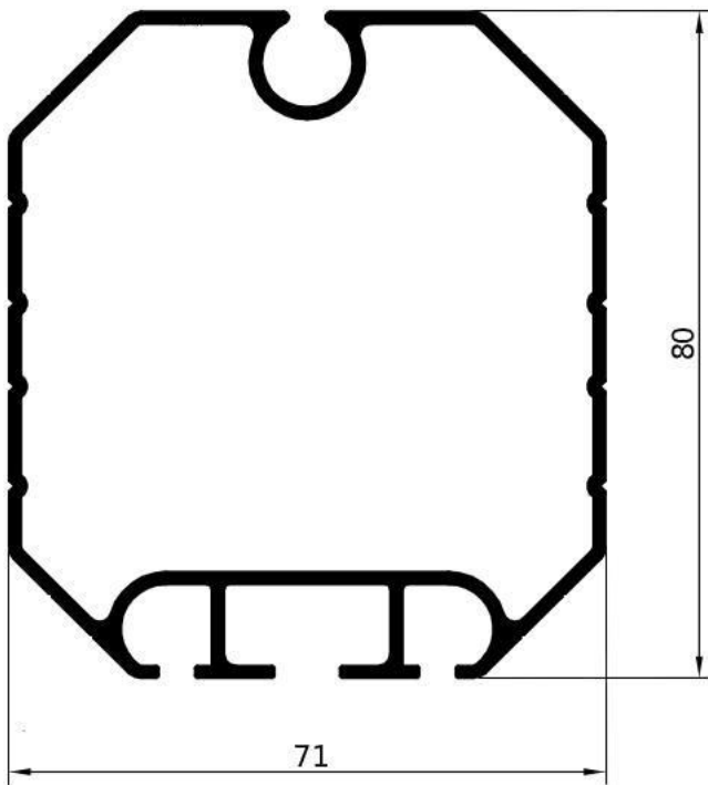
GA1522 – gr/ml 1250 L/mm.7000 PACCO / 2 BARRE
