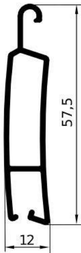
GA1514 – gr/ml 351 L/mm.6000 PACCO / 5 BARRE
