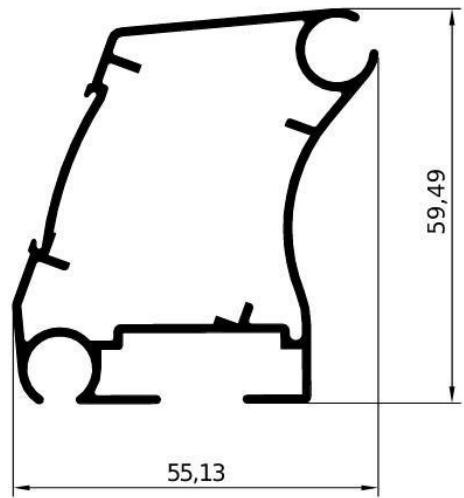
GA1669 – gr/ml 886 L/mm. 4000-5000 6000-7000 PACCO / 2 BARRE
