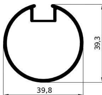
GA1002 – gr/ml 530 L/mm.7000 PACCO / 5 BARRE
