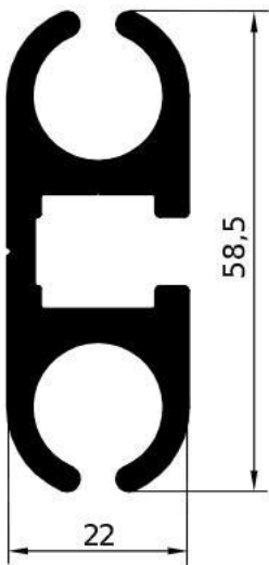
GA1526 – gr/ml 1479 L/mm.7000 PACCO / 4 BARRE
