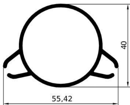
GA1513 – gr/ml 609 L/mm.7000 PACCO / 5 BARRE
