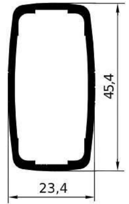
GA1507 – gr/ml 581 L/mm. 7000 PACCO / 2 BARRE
