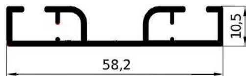
GA1574 – gr/ml 461 L/mm.6000 PACCO / 10 BARRE
