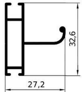
GA1533 – gr/ml 300 MIN KG.500
