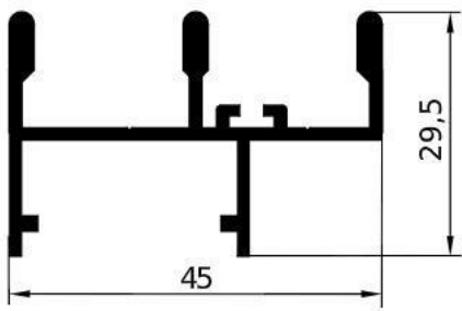
GA1536 – gr/ml 607 L/mm.6500 PACCO / 10 BARRE
