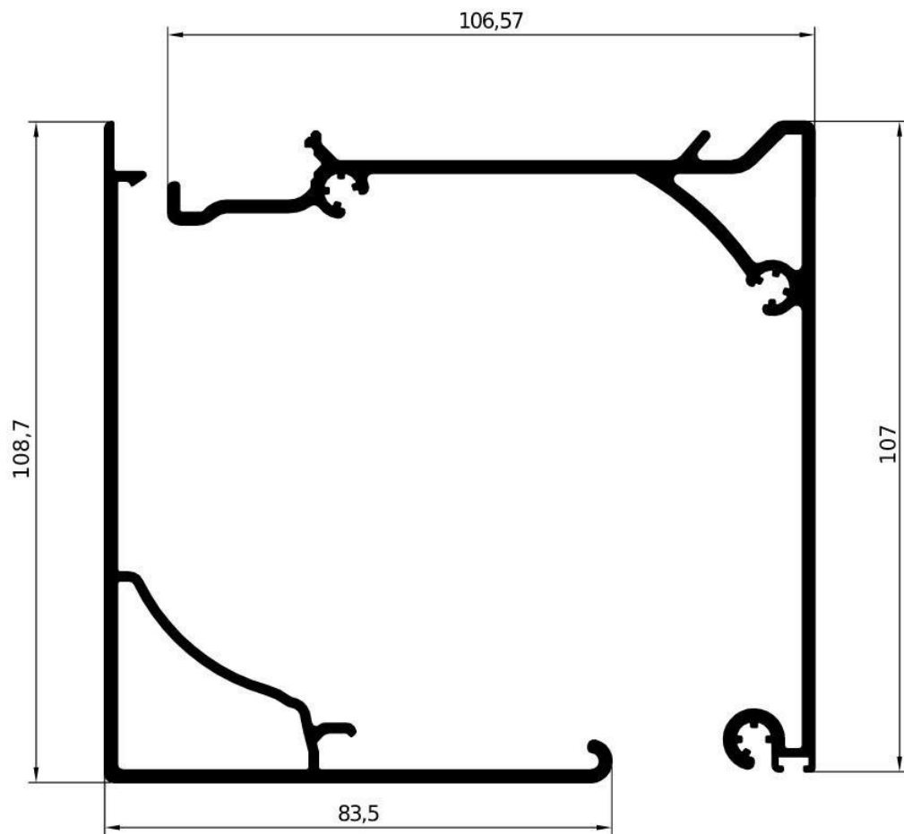
GA1683 – gr/ml 1282 CASS VEGA L/mm.7000 PACCO / 1 BARRA
