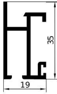
GA1537 – gr/ml 424 L/mm.6500 PACCO / 10 BARRE
