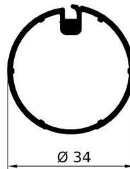
GA1654 – gr/ml 400 L/mm.6000 PACCO / 5 BARRE
