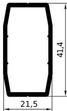
GA1677 – gr/ml 450 L/mm.6000 PACCO / 5 BARRE
