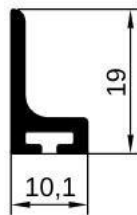
GA1665 – gr/ml 165 L/mm.6500 PACCO / 10 BARRE
