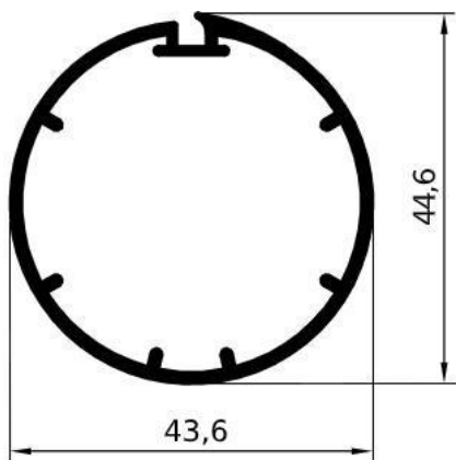
GA1636 – gr/ml 545 L/mm.6000 PACCO / 5 BARRE
